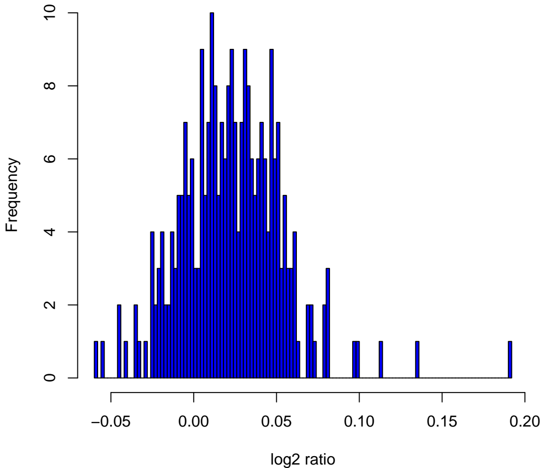
Histogram of log2ratios in 270 HapMap samples at clone Chr8tp-20D2
