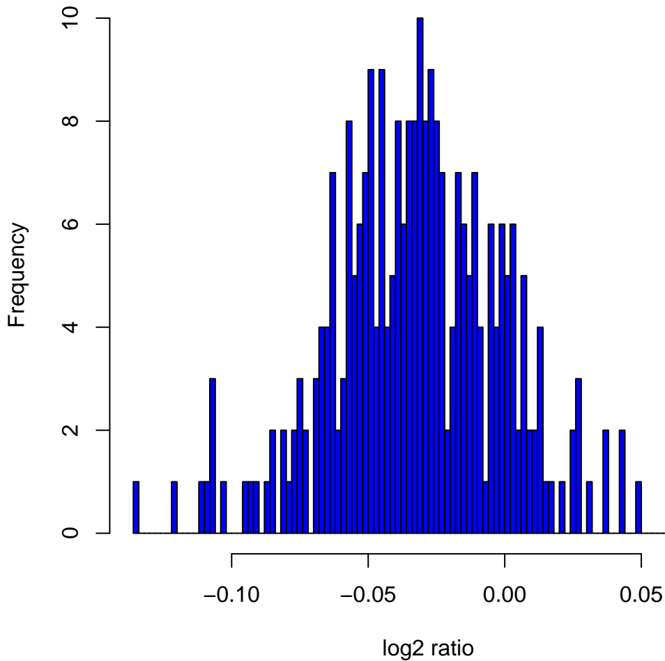
Histogram of \log_2 ratios in 270 HapMap samples at clone Chr8tp-20E2
