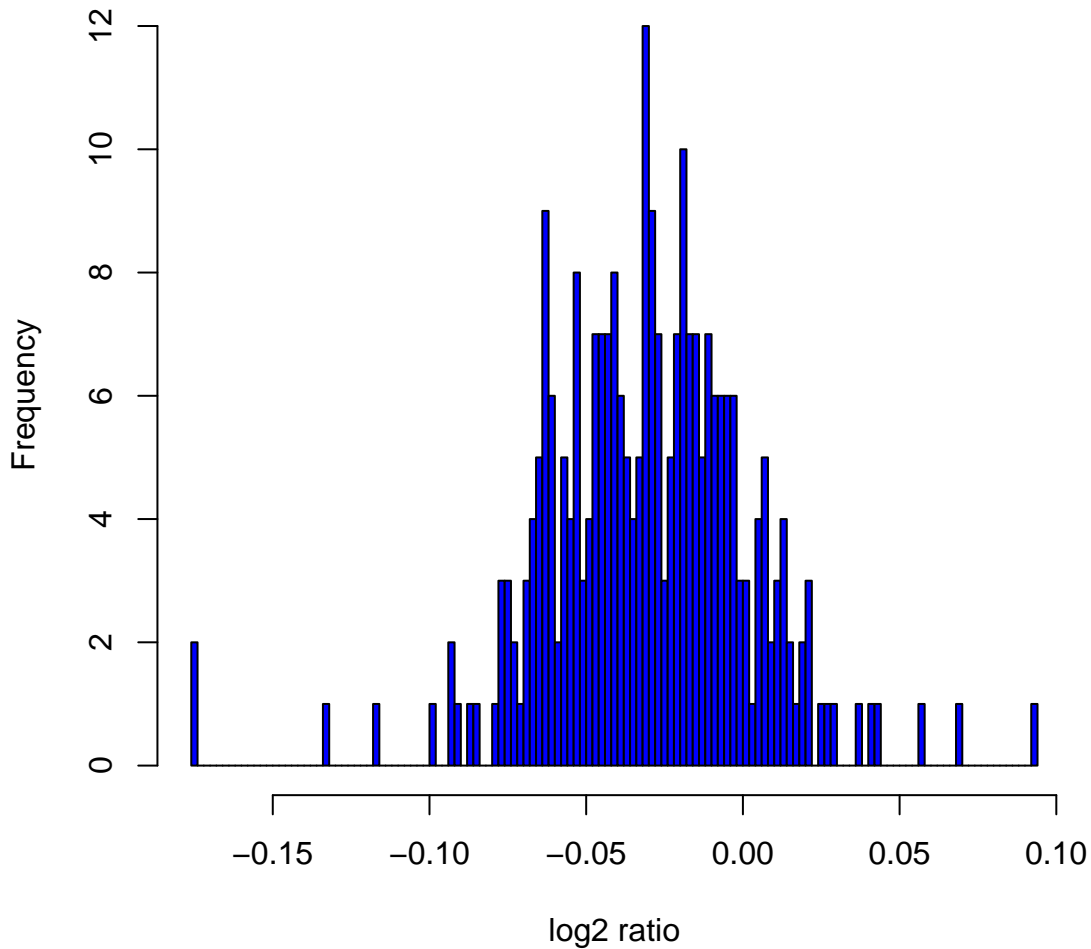
Histogram of log 2 ratios in 270 HapMap samples at clone Chr8tp-20G5
