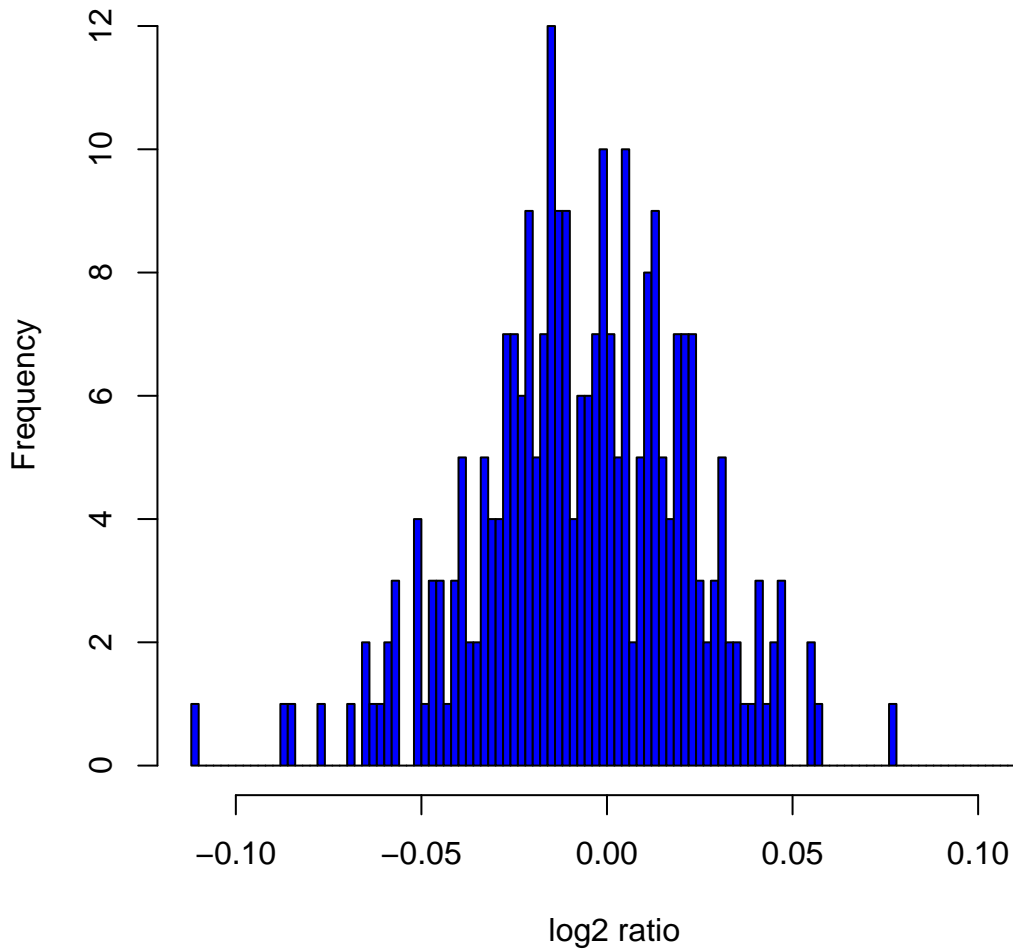
Histogram of log 2 ratios in 270 HapMap samples at clone Chr8tp-20H4
