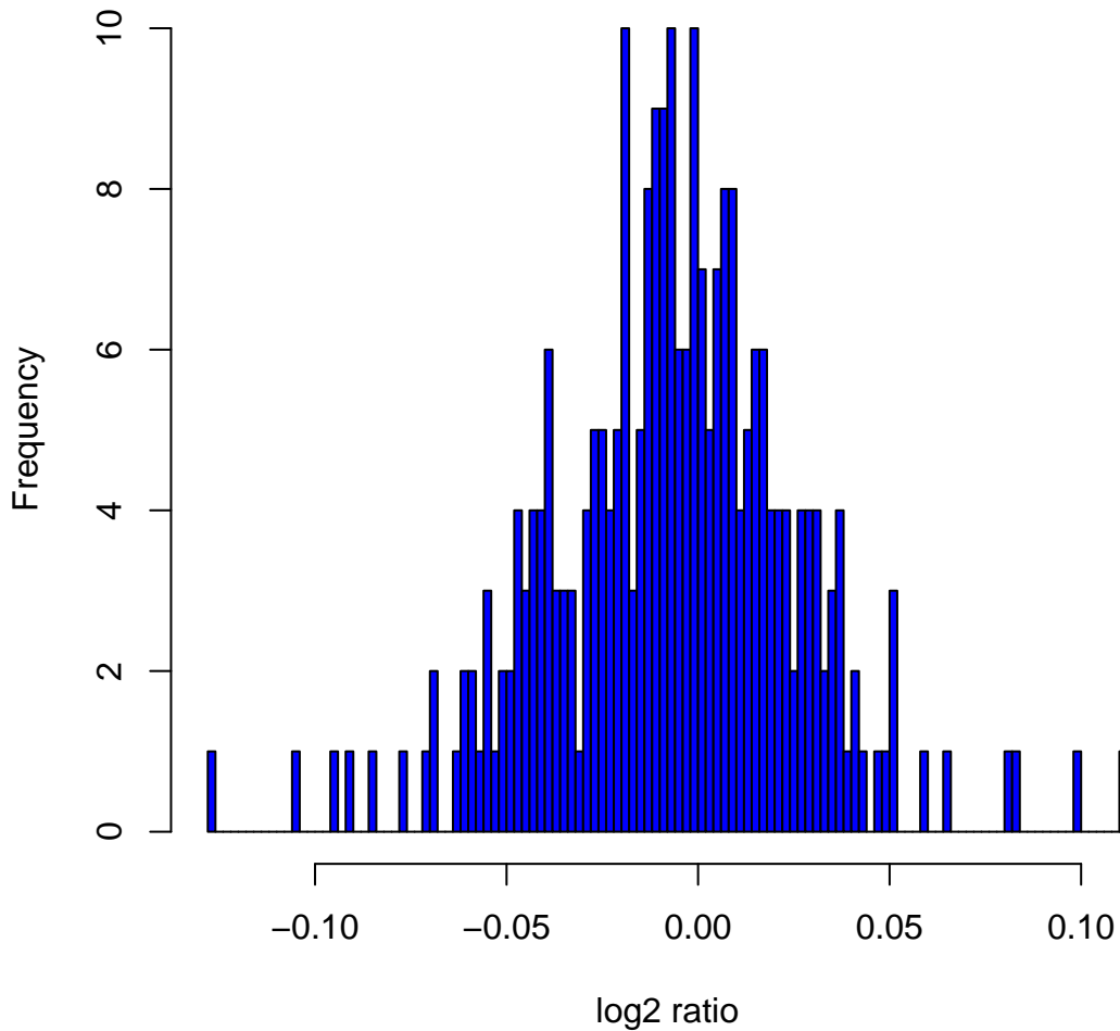
Histogram of log 2 ratios in 270 HapMap samples at clone Chr8tp-21C3
