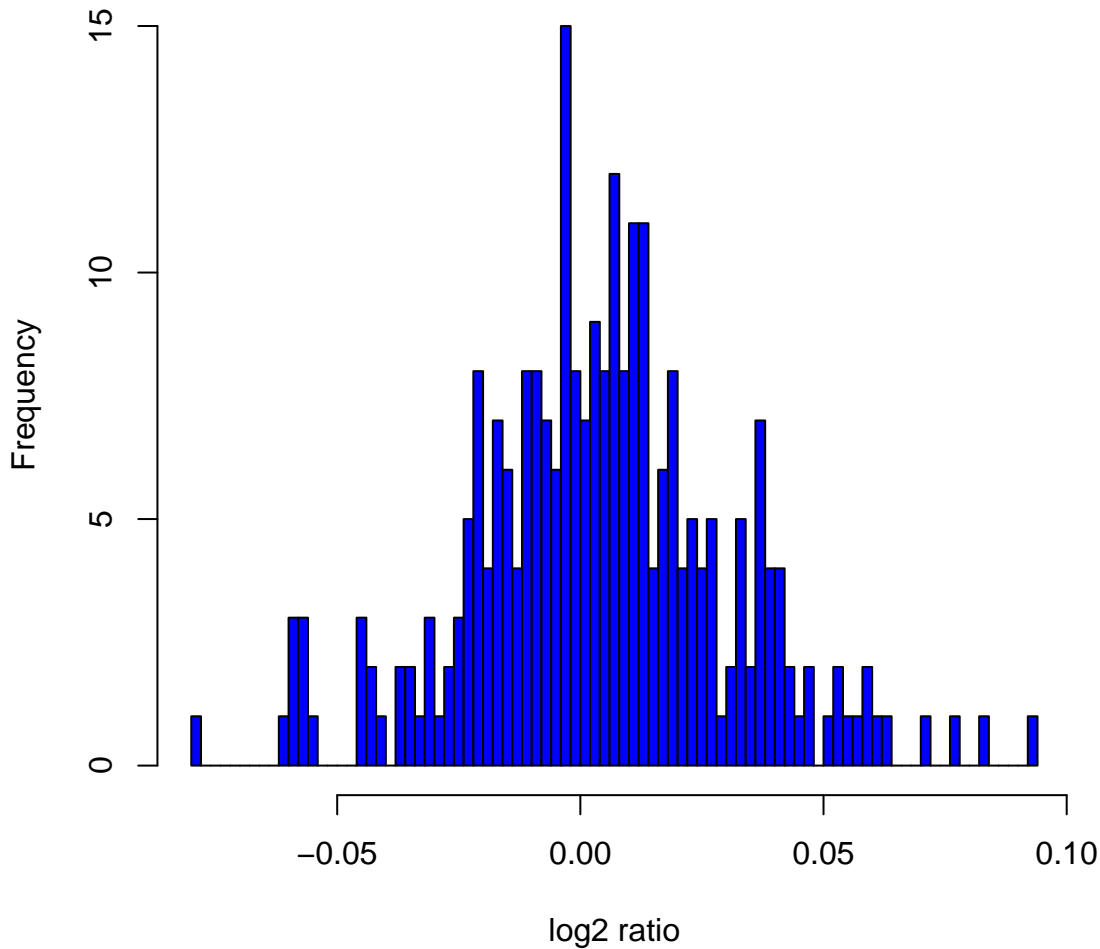
Histogram of \log_2 ratios in 270 HapMap samples at clone Chr8tp-2B11
