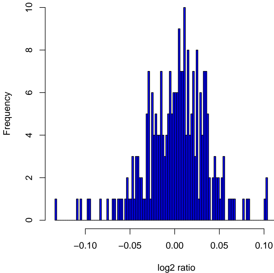
Histogram of log 2 ratios in 270 HapMap samples at clone Chr8tp-2B7
