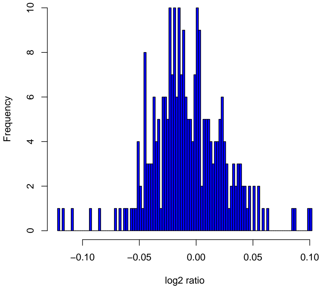
Histogram of log 2 ratios in 270 HapMap samples at clone Chr8tp-2D1
