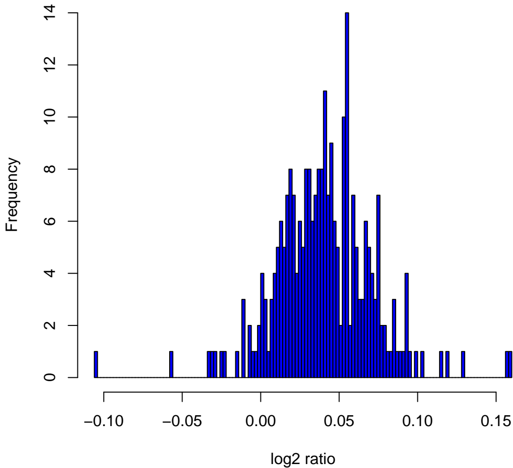
Histogram of log2ratios in 270 HapMap samples at clone Chr8tp-2F3
