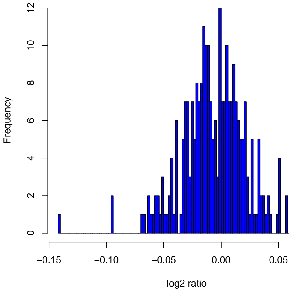
Histogram of \log_2 ratios in 270 HapMap samples at clone Chr8tp-2G9
