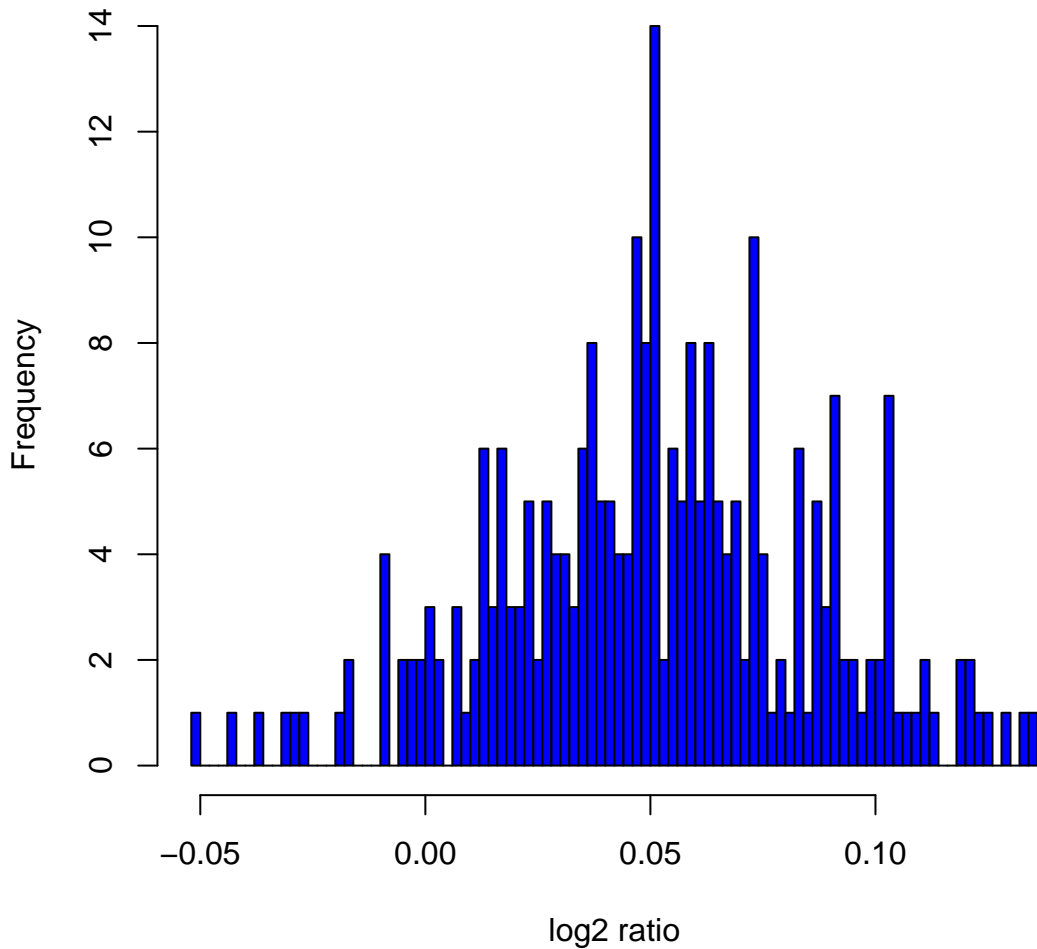
Histogram of log 2 ratios in 270 HapMap samples at clone Chr8tp-2H2
