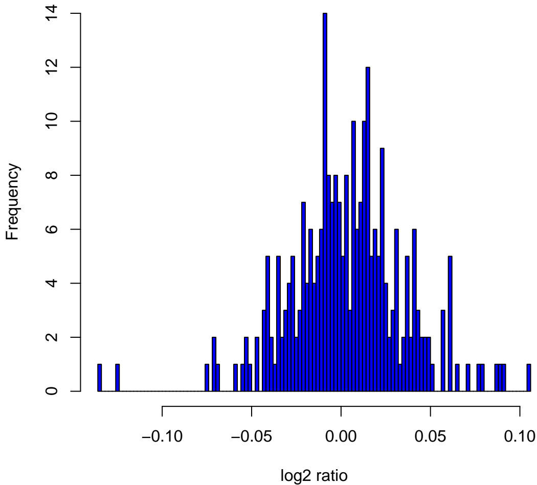
Histogram of \log_2 ratios in 270 HapMap samples at clone Chr8tp-2H4
