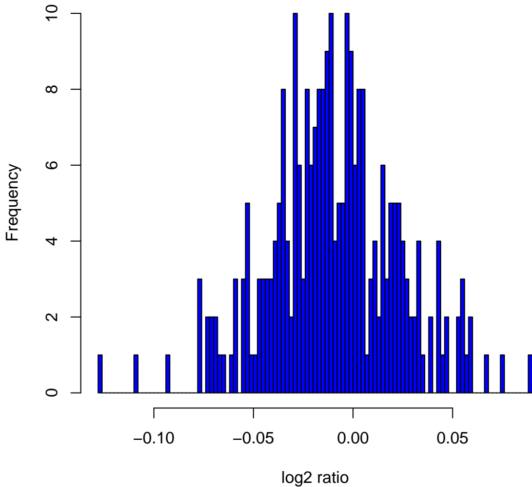
Histogram of \log_2 ratios in 270 HapMap samples at clone Chr8tp-2H5
