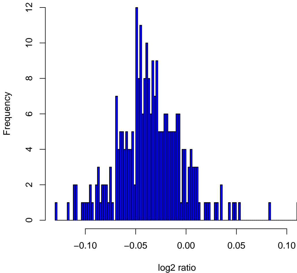
Histogram of log 2 ratios in 270 HapMap samples at clone Chr8tp-3A10
