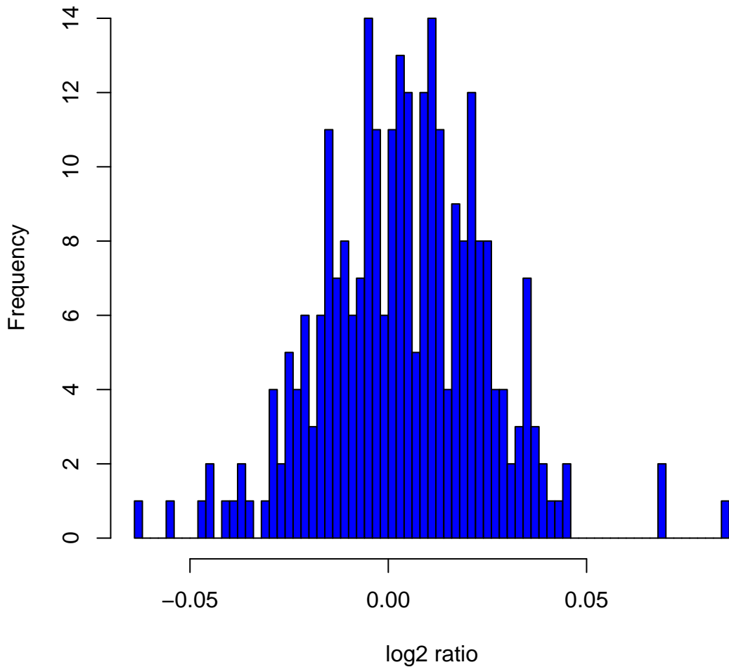
Histogram of \log_2 ratios in 270 HapMap samples at clone Chr8tp-3A5
