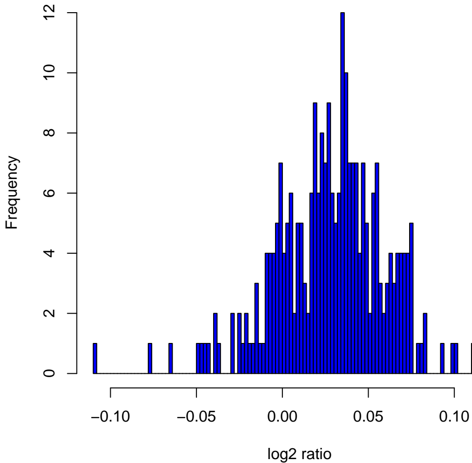
Histogram of log 2 ratios in 270 HapMap samples at clone Chr8tp-3D2
