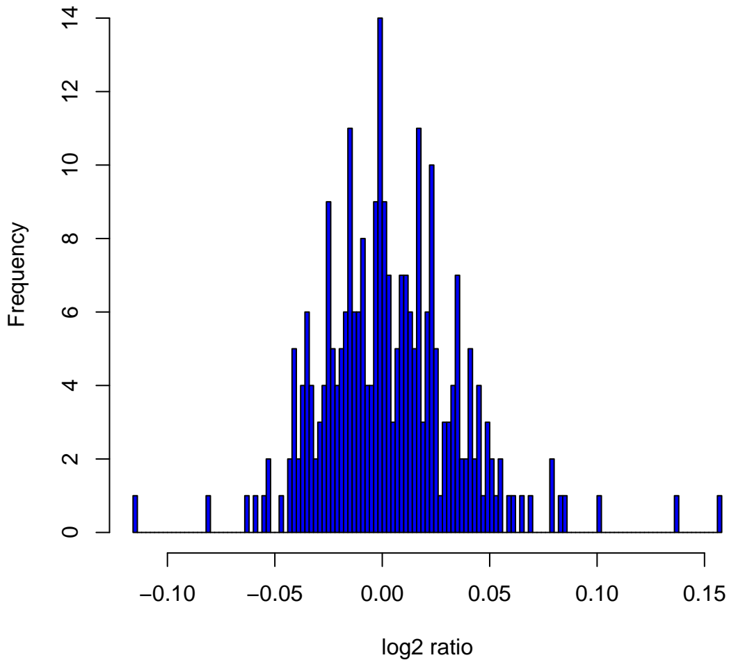
Histogram of log2ratios in 270 HapMap samples at clone Chr8tp-3E2
