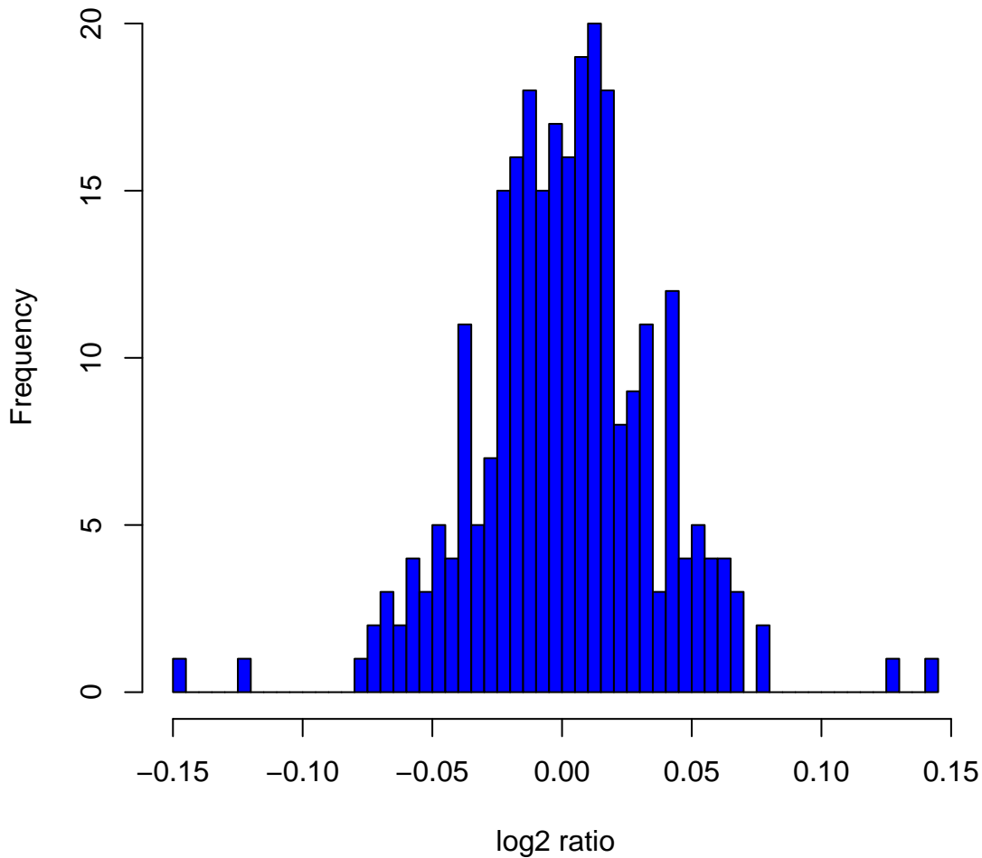
Histogram of log 2 ratios in 270 HapMap samples at clone Chr8tp-3E9
