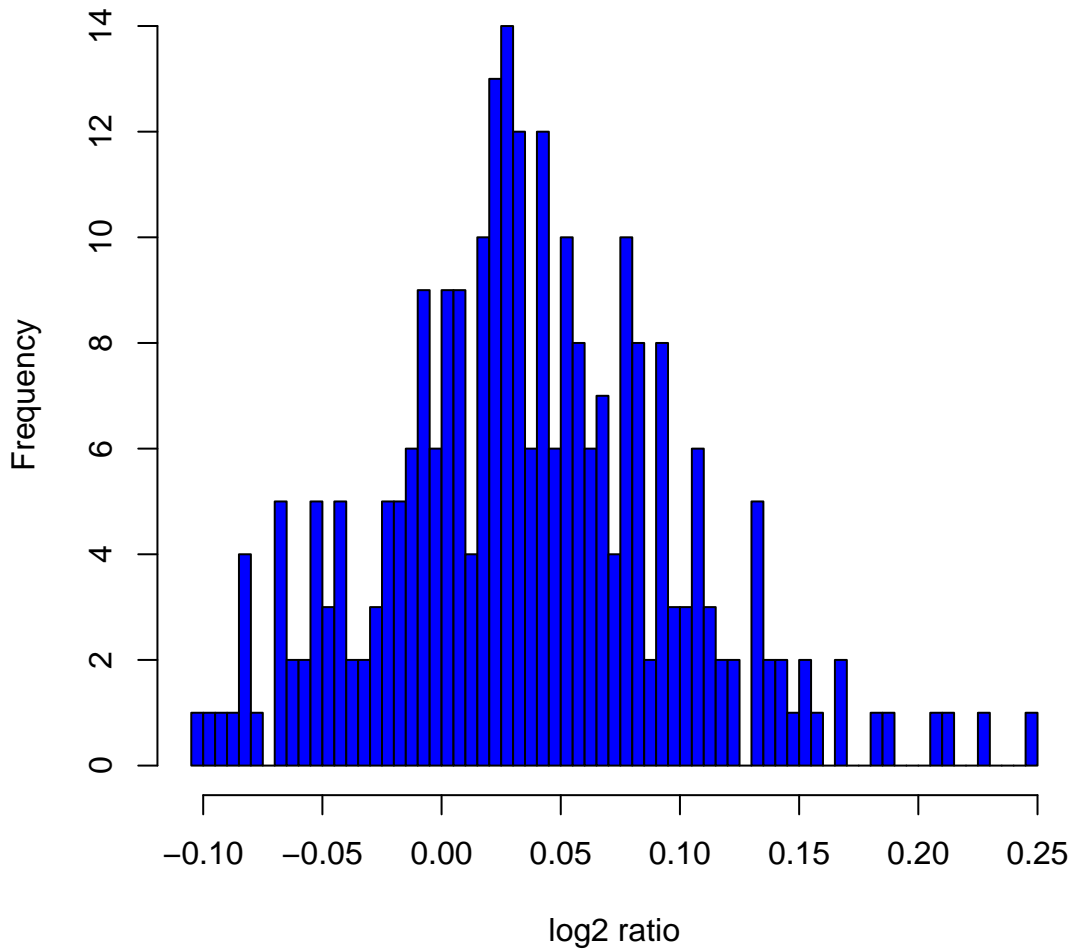
Histogram of log 2 ratios in 270 HapMap samples at clone Chr8tp-3F4
