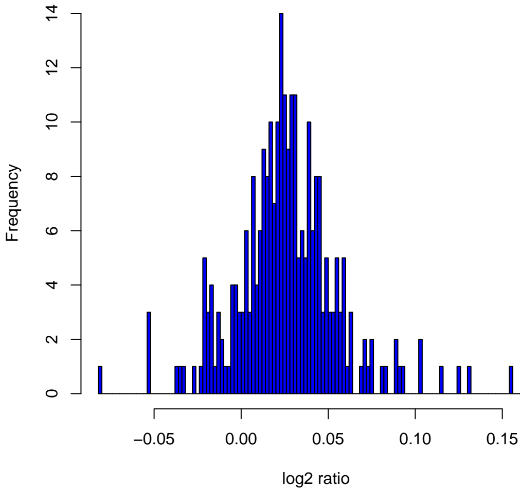
Histogram of log 2 ratios in 270 HapMap samples at clone Chr8tp-3G3
