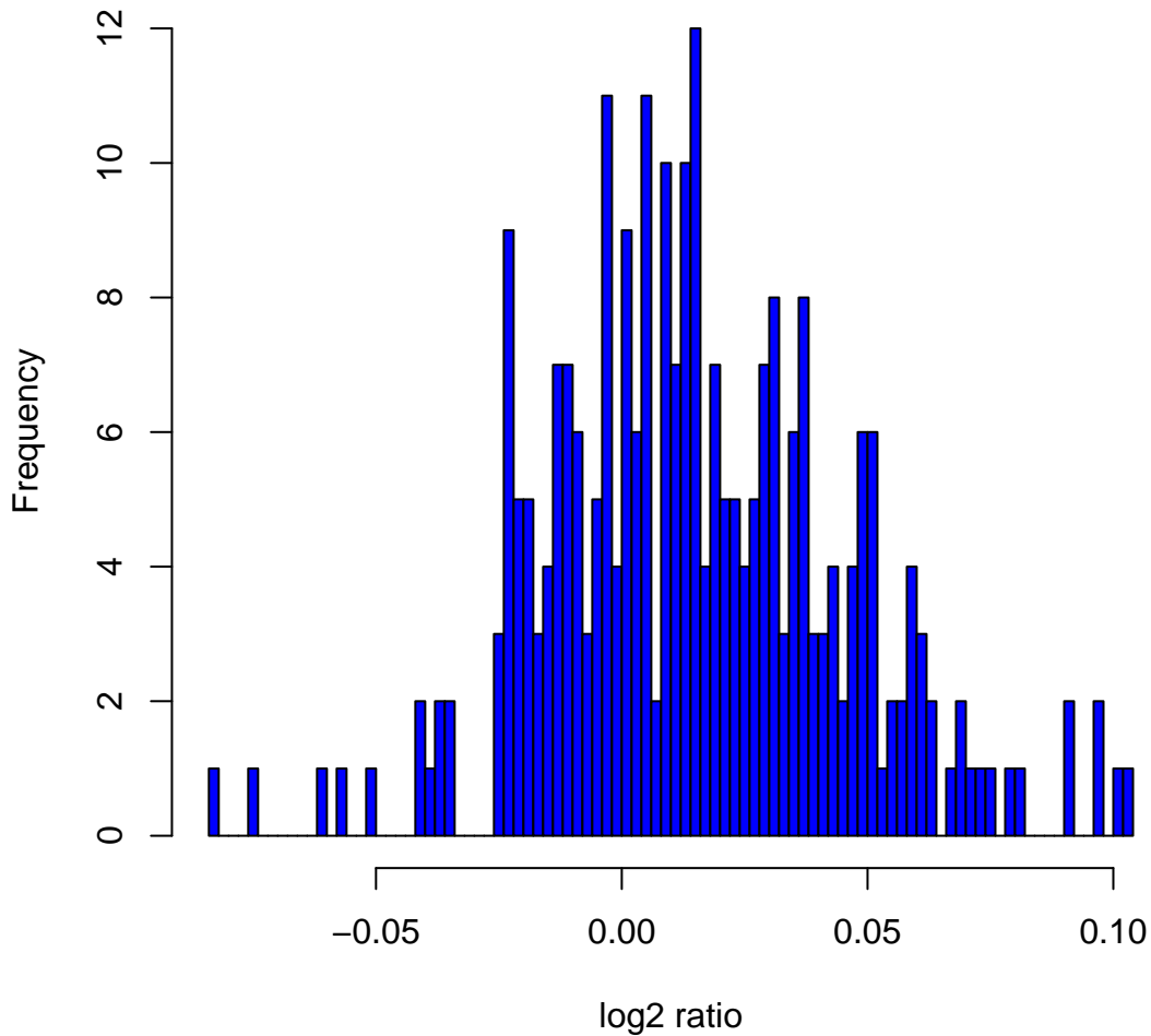
Histogram of log 2 ratios in 270 HapMap samples at clone Chr8tp-4A4
