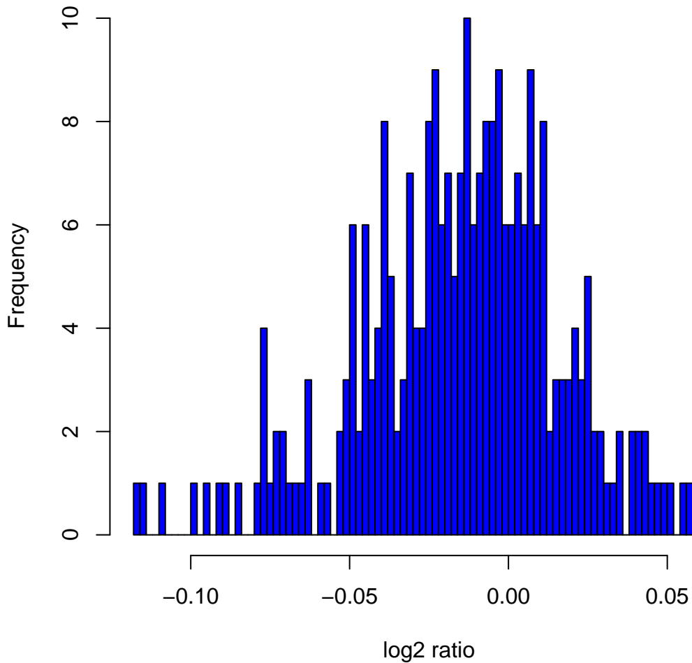
Histogram of log 2 ratios in 270 HapMap samples at clone Chr8tp-4A7
