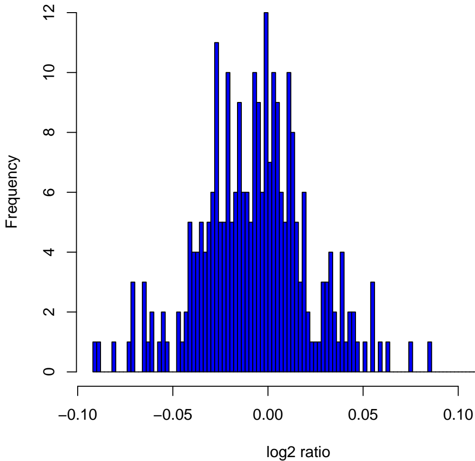
Histogram of \log_2 ratios in 270 HapMap samples at clone Chr8tp-4B4
