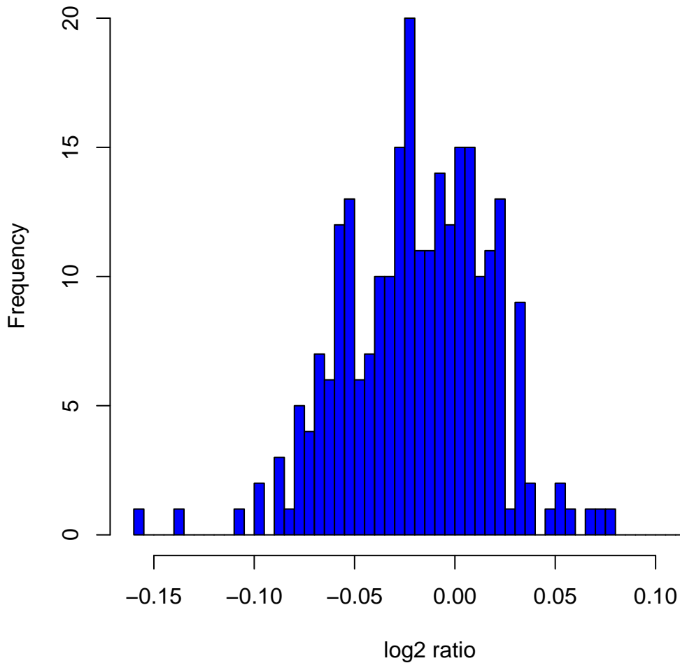
Histogram of log 2 ratios in 270 HapMap samples at clone Chr8tp-4B6
