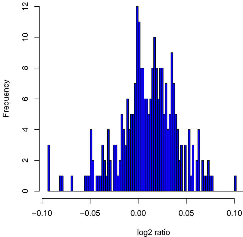
Histogram of log 2 ratios in 270 HapMap samples at clone Chr8tp-4C4
