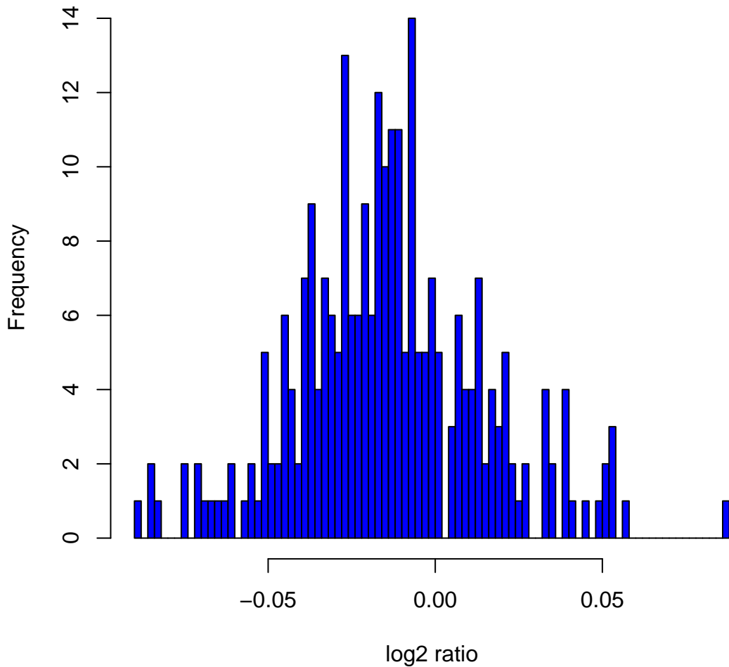
Histogram of log2ratios in 270 HapMap samples at clone Chr8tp-4E1
