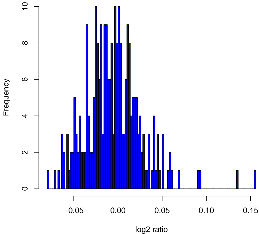
Histogram of log 2 ratios in 270 HapMap samples at clone Chr8tp-4E11
