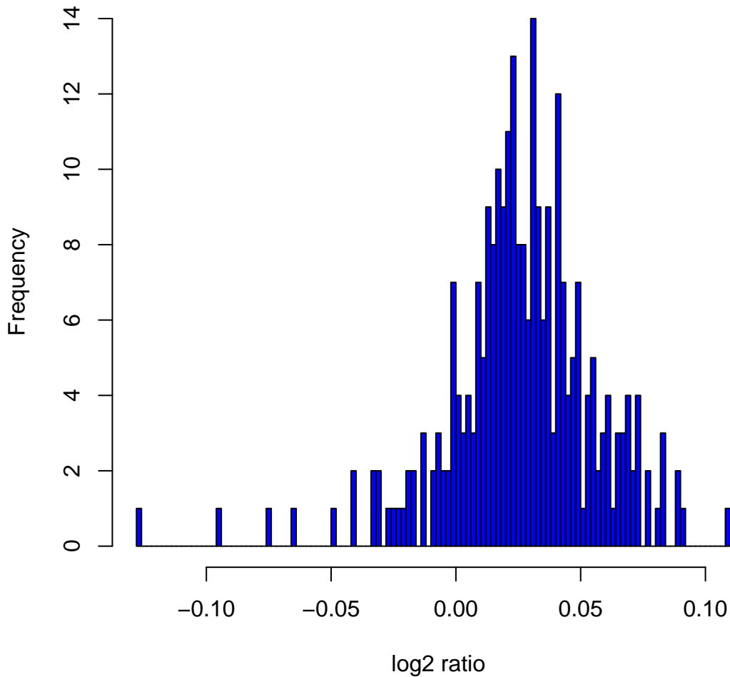
Histogram of log 2 ratios in 270 HapMap samples at clone Chr8tp-4E9
