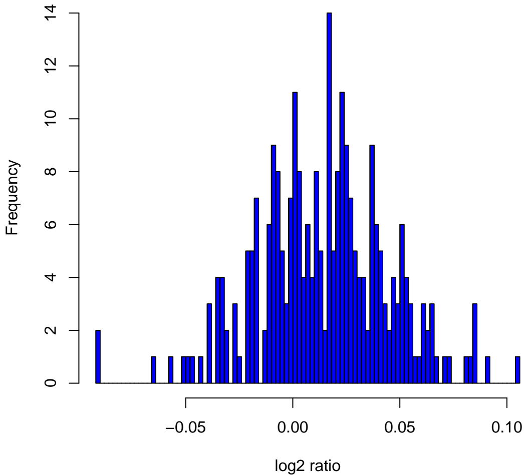
Histogram of log 2 ratios in 270 HapMap samples at clone Chr8tp-4G5
