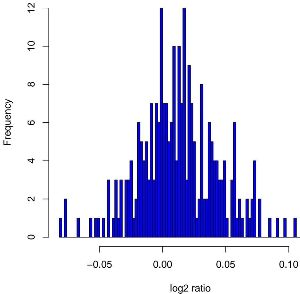
Histogram of log 2 ratios in 270 HapMap samples at clone Chr8tp-4H6
