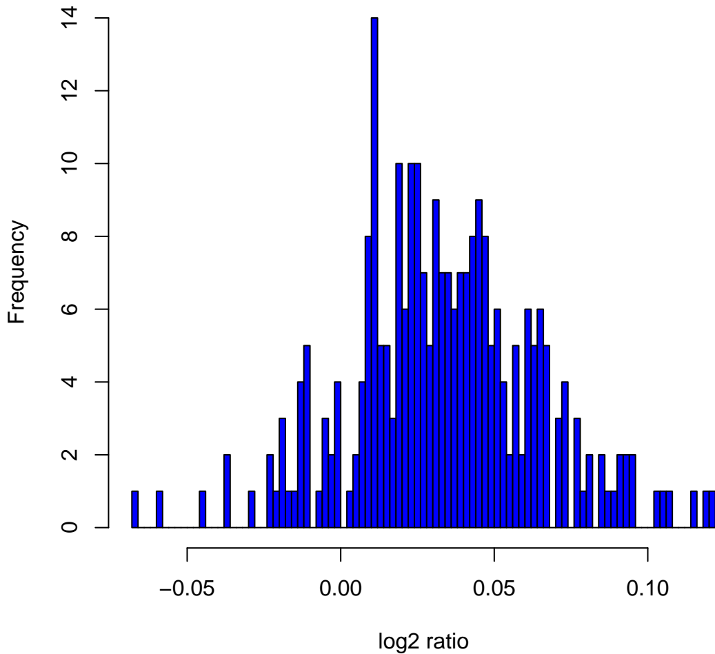
Histogram of \log_2 ratios in 270 HapMap samples at clone Chr8tp-5B3
