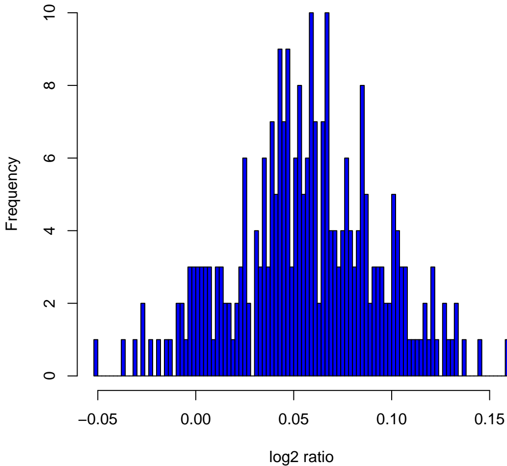
Histogram of log 2 ratios in 270 HapMap samples at clone Chr8tp-5B6
