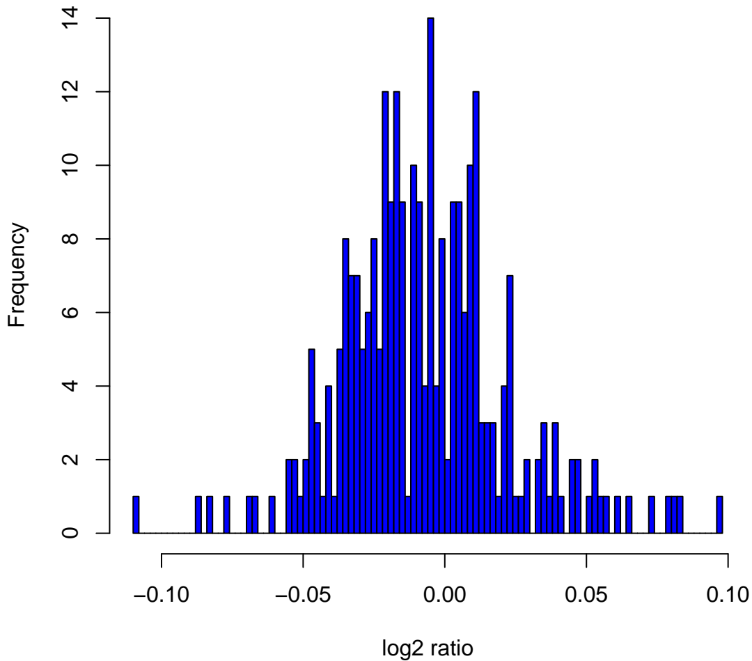
Histogram of log 2 ratios in 270 HapMap samples at clone Chr8tp-5E3
