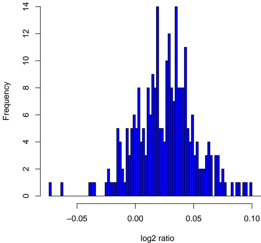
Histogram of log2ratios in 270 HapMap samples at clone Chr8tp-5E4
