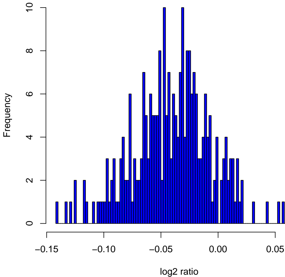
Histogram of \log_2 ratios in 270 HapMap samples at clone Chr8tp-5E5
