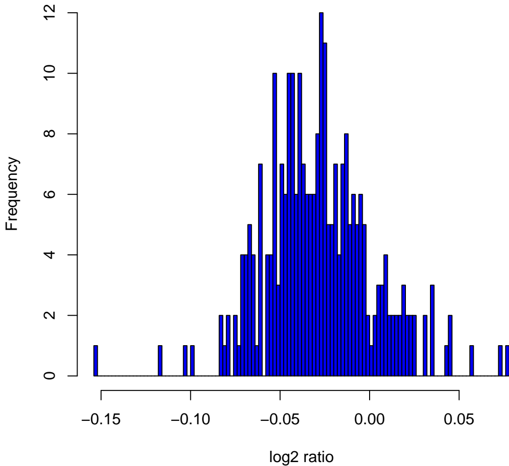
Histogram of log 2 ratios in 270 HapMap samples at clone Chr8tp-5G2
