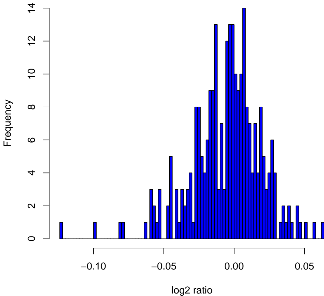
Histogram of log 2 ratios in 270 HapMap samples at clone Chr8tp-5G3
