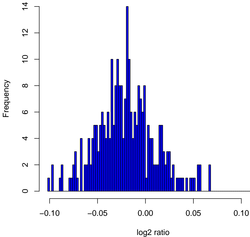
Histogram of log 2 ratios in 270 HapMap samples at clone Chr8tp-5G9
