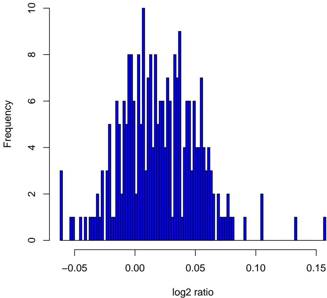
Histogram of log 2 ratios in 270 HapMap samples at clone Chr8tp-5H7
