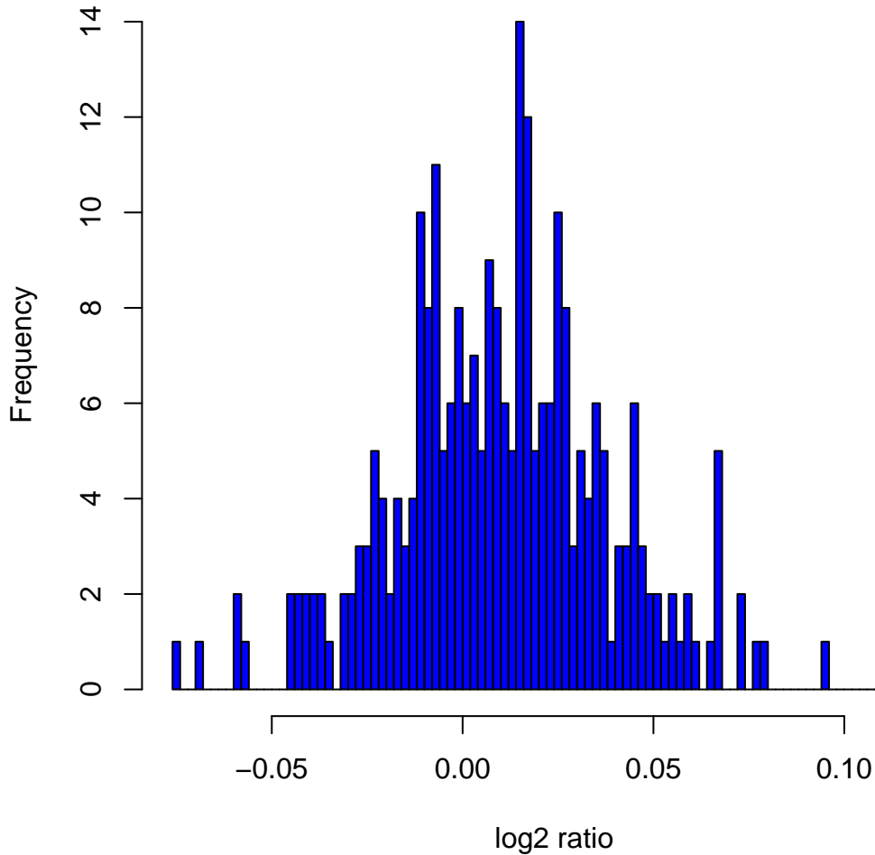
Histogram of log 2 ratios in 270 HapMap samples at clone Chr8tp-6B11
