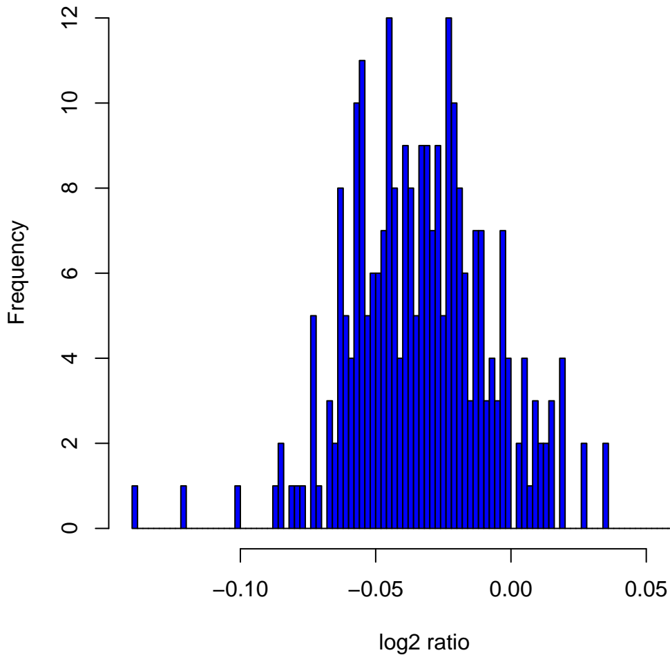
Histogram of \log_2 ratios in 270 HapMap samples at clone Chr8tp-6B6
