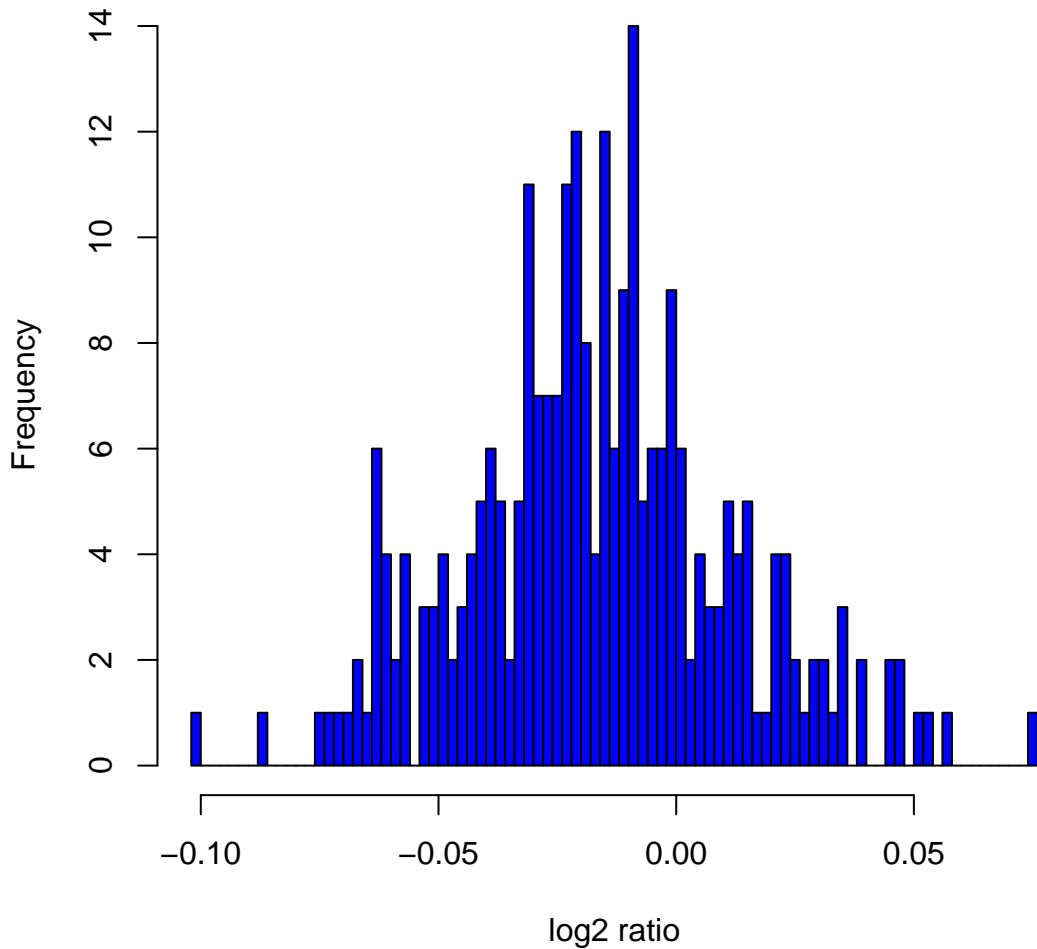
Histogram of log 2 ratios in 270 HapMap samples at clone Chr8tp-6D8
