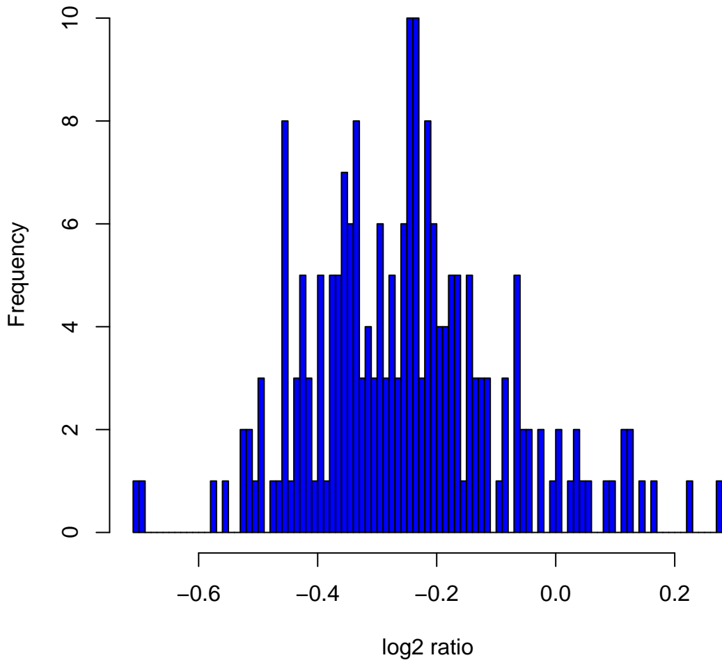
Histogram of log 2 ratios in 270 HapMap samples at clone Chr8tp-6E11
