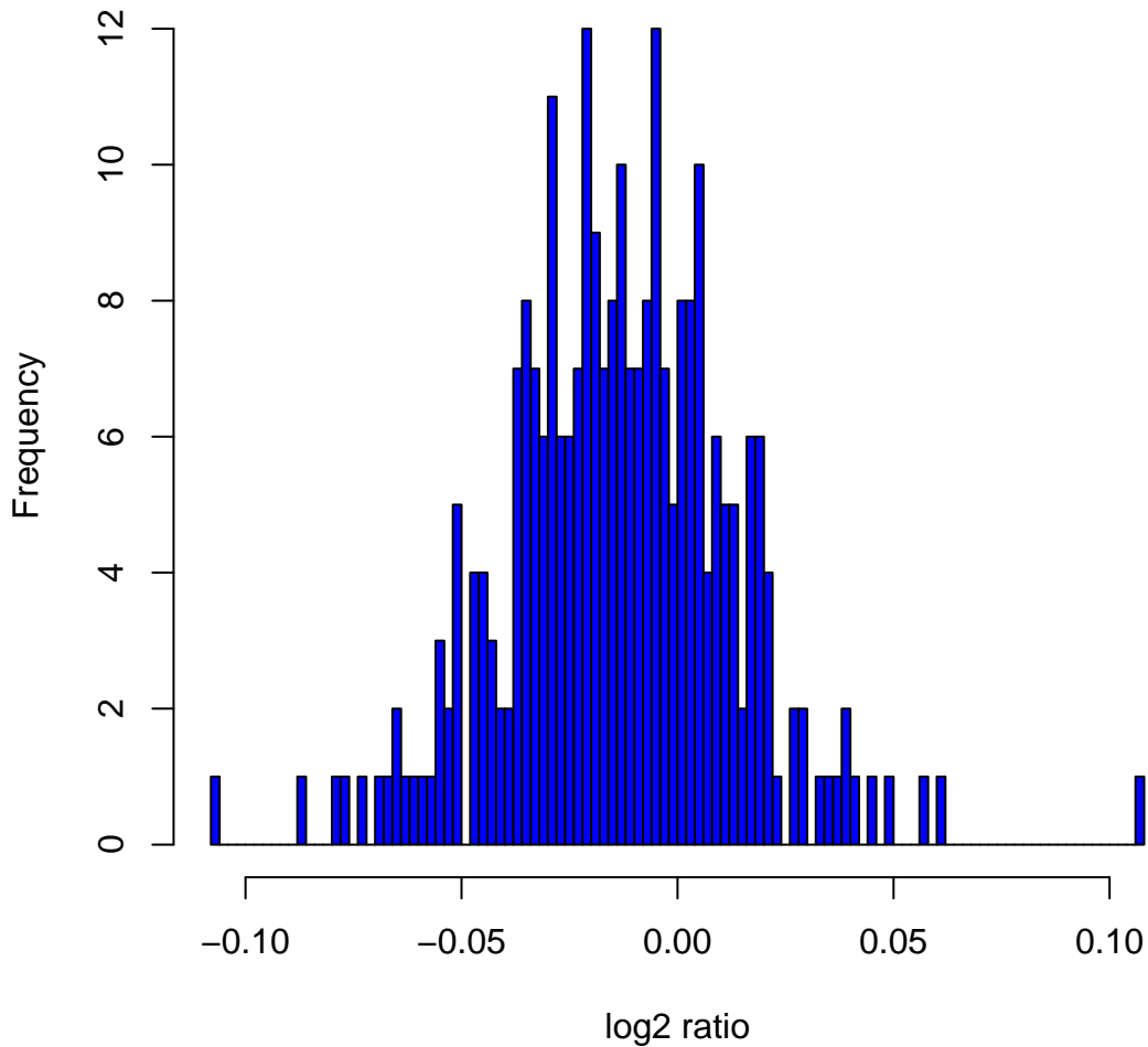
Histogram of \log_2 ratios in 270 HapMap samples at clone Chr8tp-6E2
