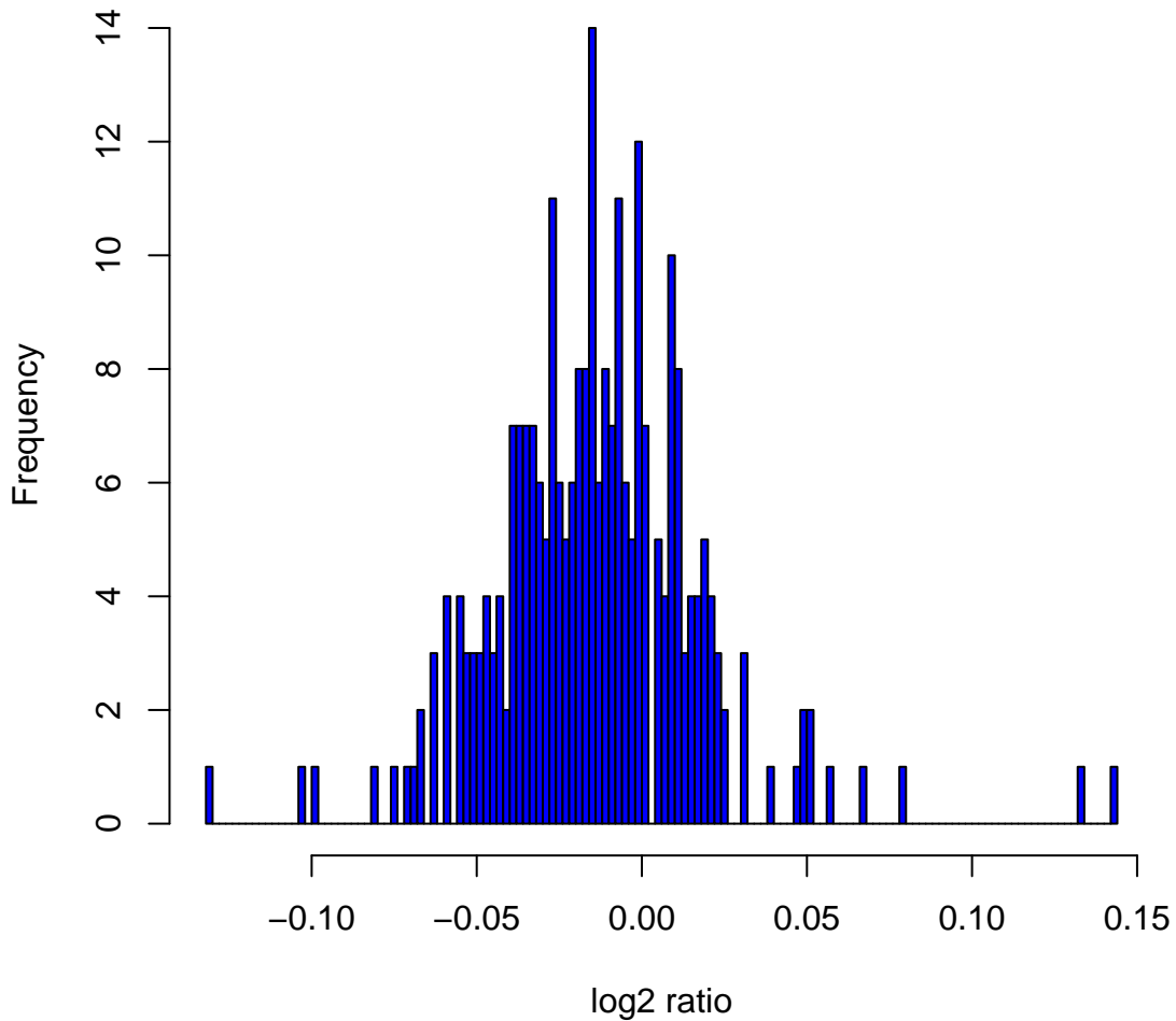
Histogram of log 2 ratios in 270 HapMap samples at clone Chr8tp-6H9
