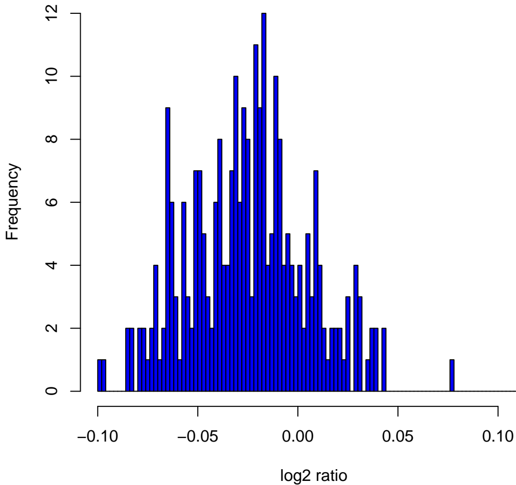
Histogram of \log_2 ratios in 270 HapMap samples at clone Chr8tp-7A7
