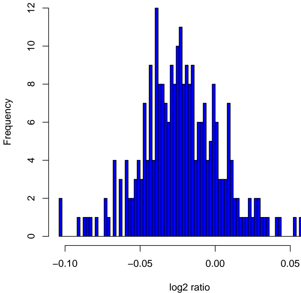
Histogram of \log_2 ratios in 270 HapMap samples at clone Chr8tp-7B2
