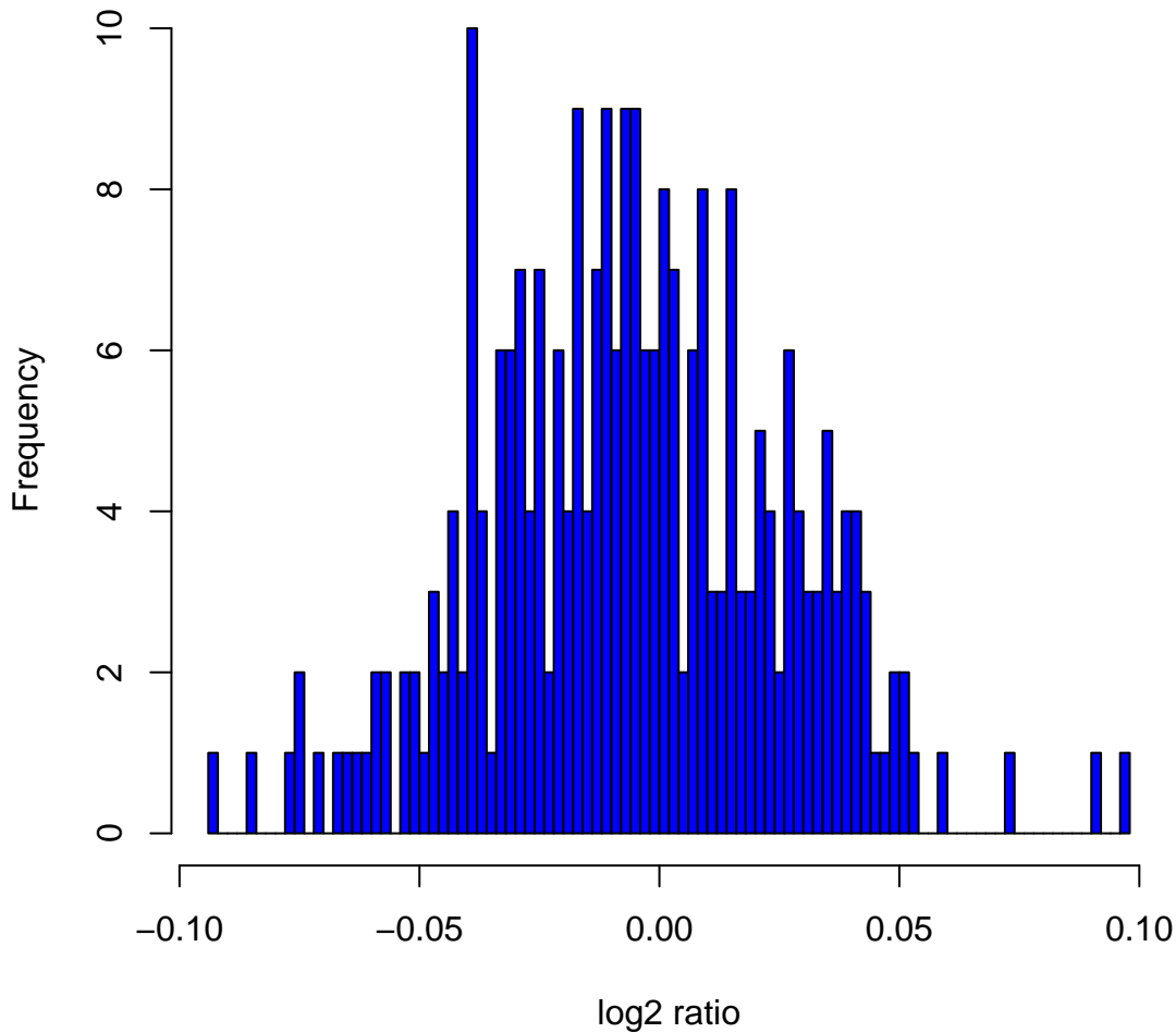
Histogram of \log_2 ratios in 270 HapMap samples at clone Chr8tp-7B5
