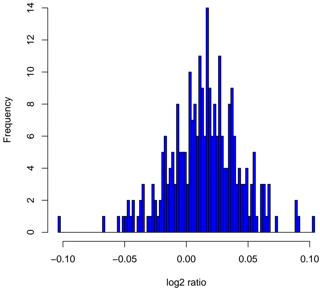
Histogram of log2ratios in 270 HapMap samples at clone Chr8tp-7B6
