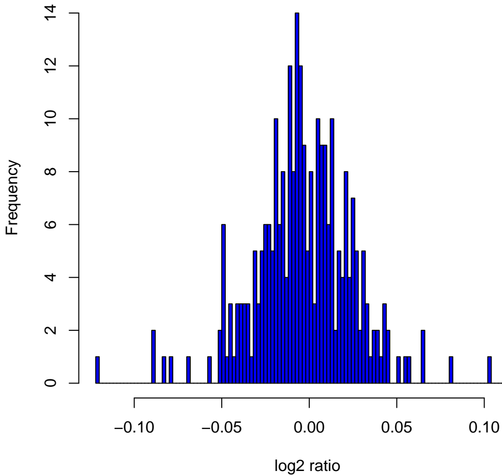
Histogram of \log_2 ratios in 270 HapMap samples at clone Chr8tp-7C5
